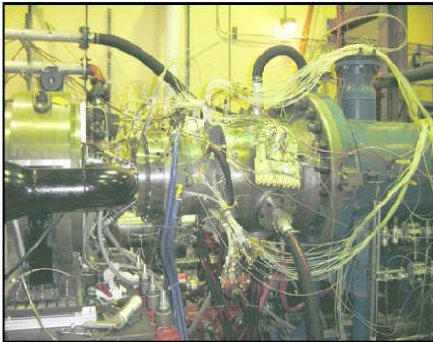
Figure 1 Rampressor-1 Test Rig Installed in Test Cell
